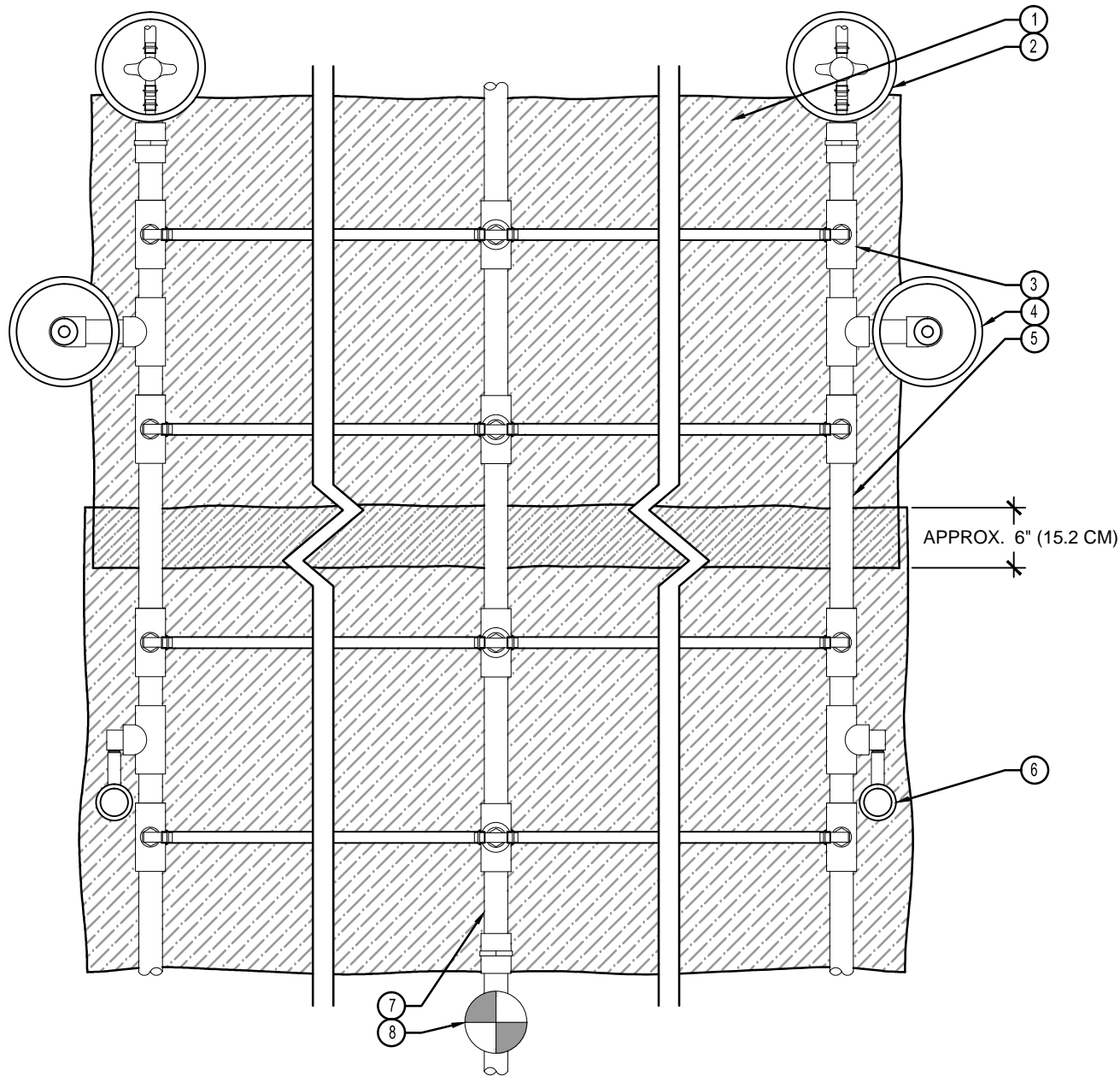
XX ECO-MAT PLAN VIEW WITH PVC HEADER AND EXHAUST CENTER FEED Hunter HM.EM.20
